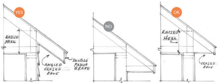
Figure 30. Gable End + Horizontal Eave Transition
