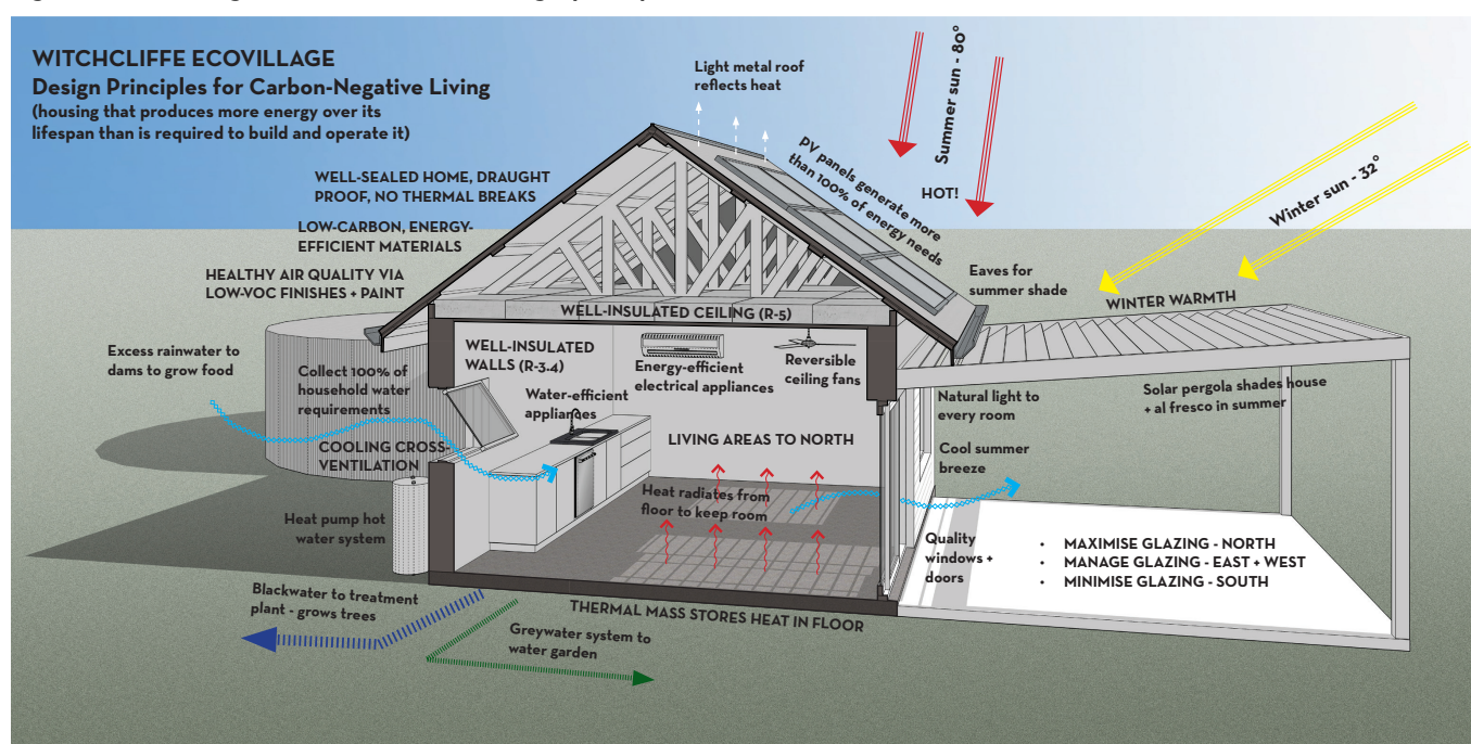
Figure 2. WEV Negative carbon house design principles
