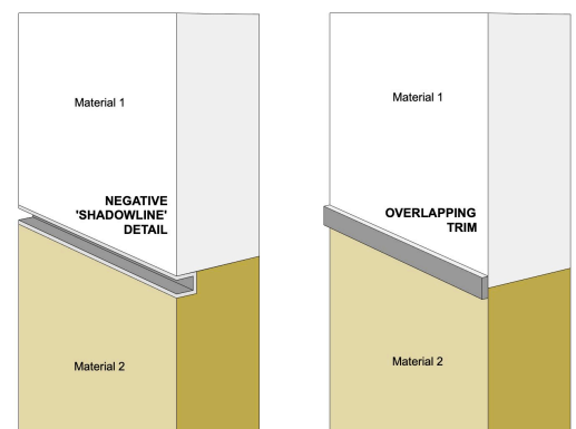
Figure 28. Horizontal colour / materials changes
